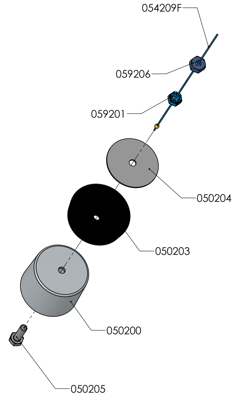
PLUNGER ASSY
