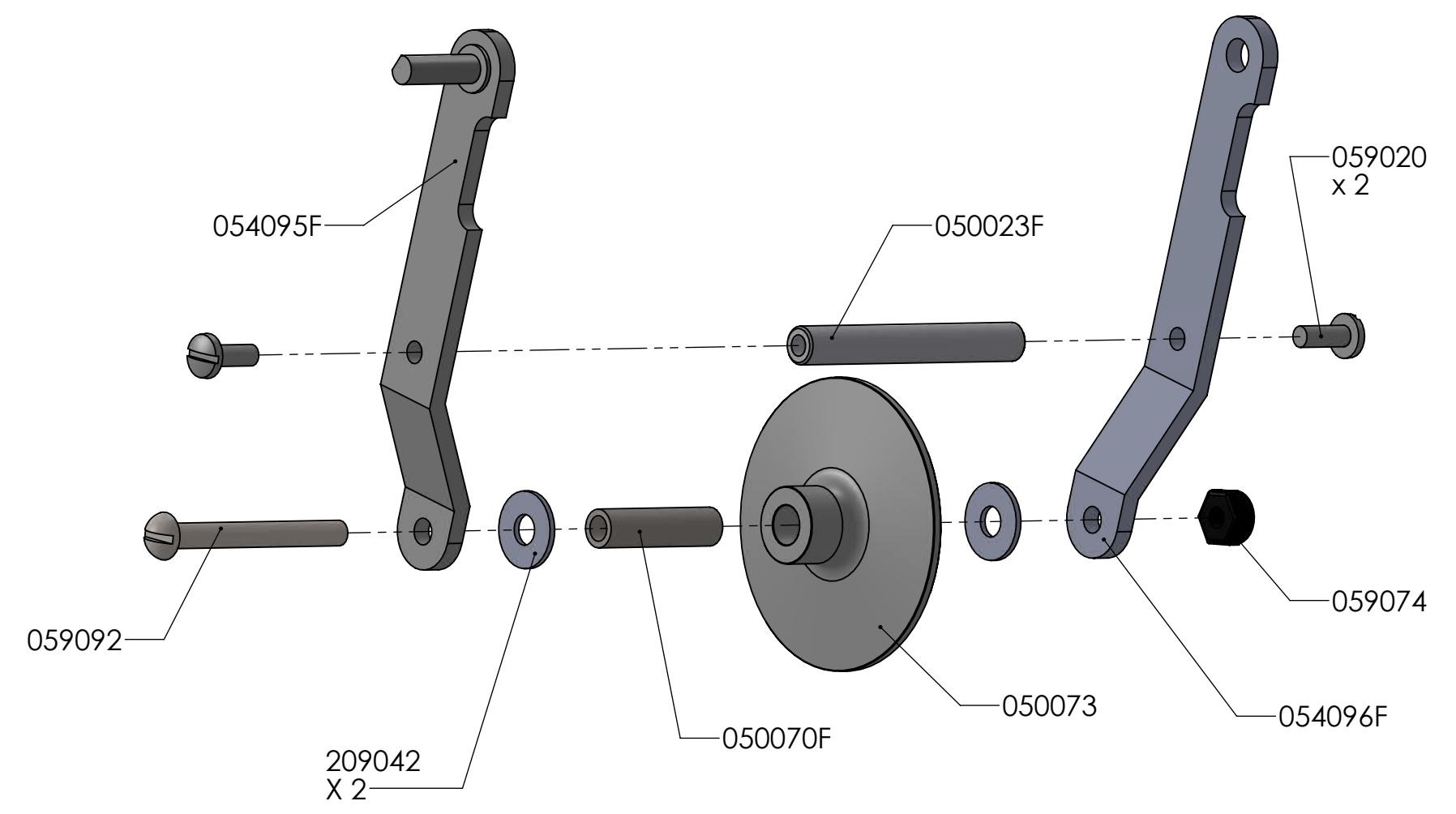
CREASER ASSY
