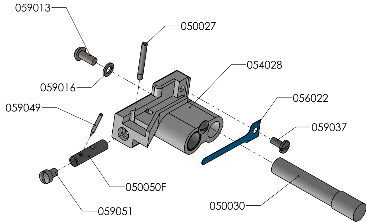
GOOSER ASSY
